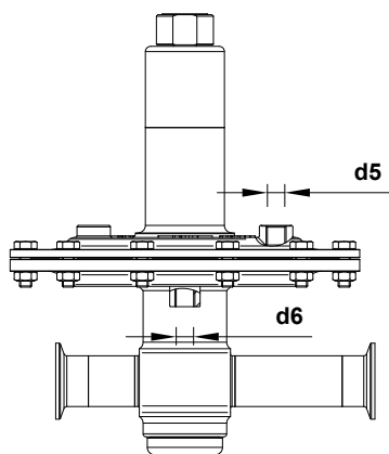
Optional external sensing and leakage line connections
