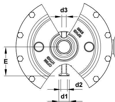
Optional gauge connection
